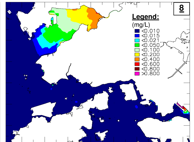
Scenario 5b (Emergency Discharge at Bypass Location)
